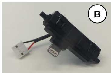
Gender Assy - Lightning
